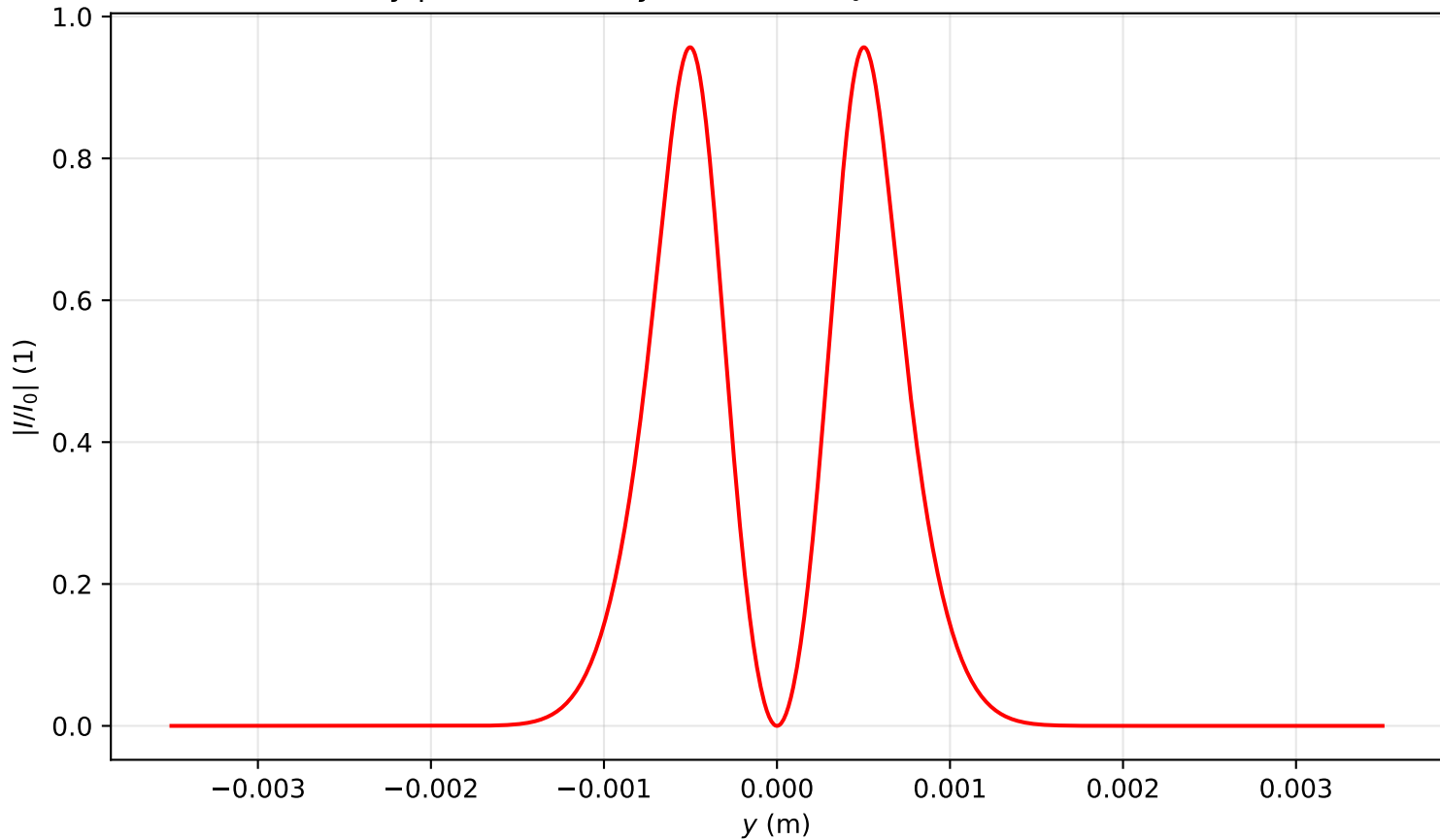
Intensity profile I(x=0, y, z=0.318)/I_0 , P_{in}=4.0P_{cr} , artificial time
